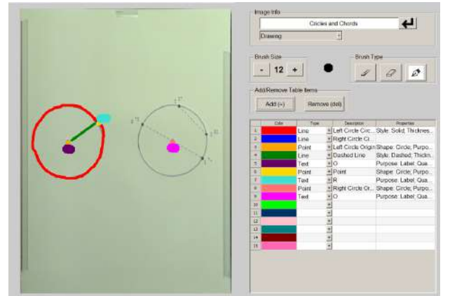
Figure 4: Annotation GUI.
